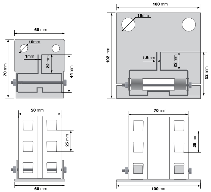
Upright M50 (with footplate) -use M8 floor fixing
