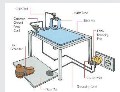
Static Dissipative System Setup
